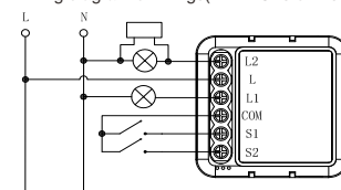
Wiring diagram of fittings(L1 L2 One of them)
