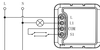
Wiring diagram of fittings(L1 L2 One of them)
