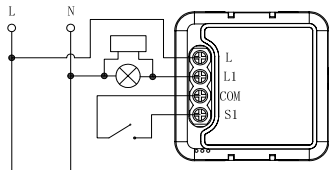
Wiring diagram of fittings
